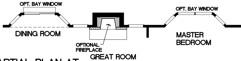
PARTIAL PLAN AT OPT. BAY WINDOW
