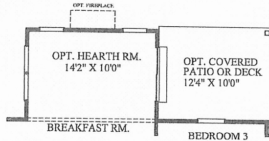
PARTIAL FIRST FLOOR PLAN OPTIONAL HEARTH ROOM
