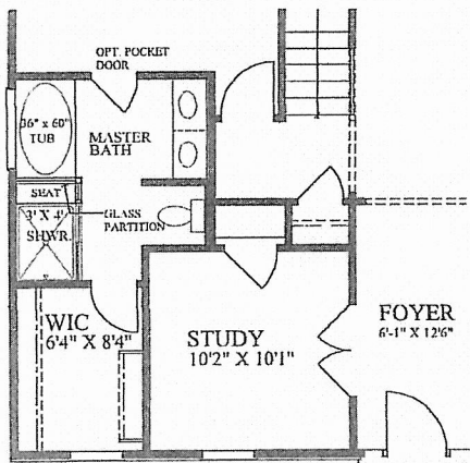
PARTIAL FIRST FLOOR PLAN OPTIONAL STUDY & OPT. LUXURY BATH
