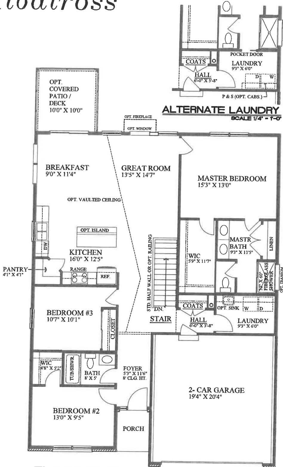
FLOOR PLAN 1569 S.F.
